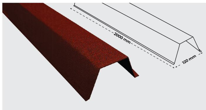
Flat Ridge Cap 2000 x 120 mm
