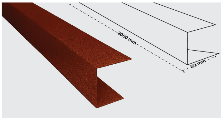
U Shape Valley 2000 x 152 mm
